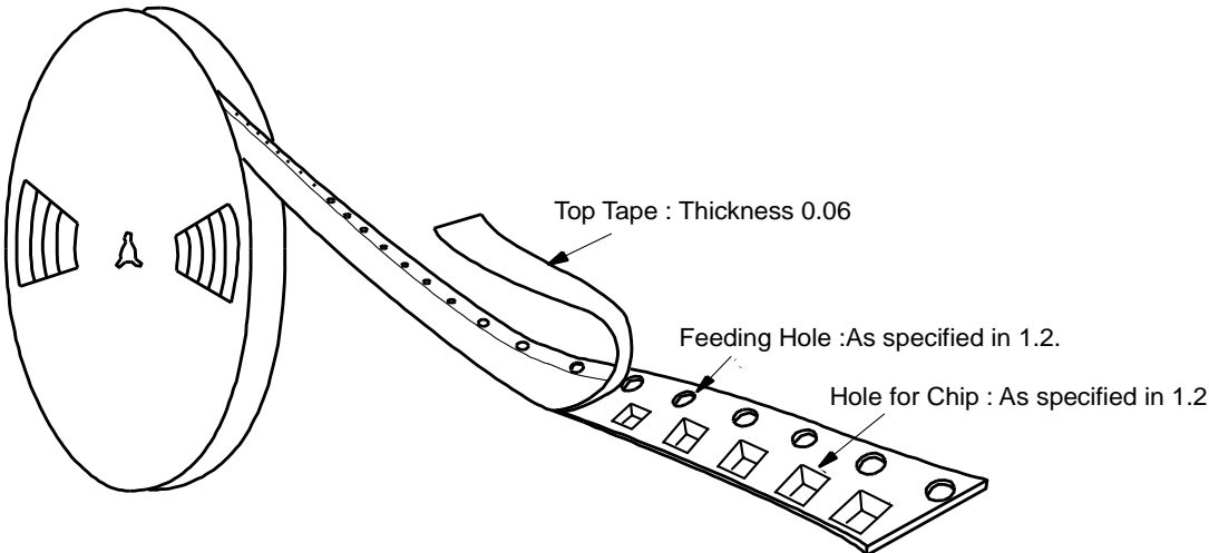
Fig.3 Taping Diagram
